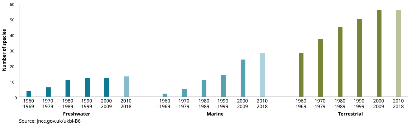
UK Biodiversity Indicator: Number of new INNS established in or along 10% or more of Great Britain’s land area or coastline, 1960 to 2018 (final columns in each habitat refer to nine years rather than 10)
