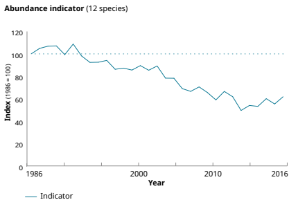
Index of seabird numbers in Scotland, 1986 to 2016
